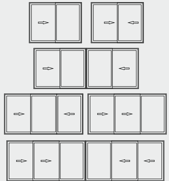
Sliding Windows
